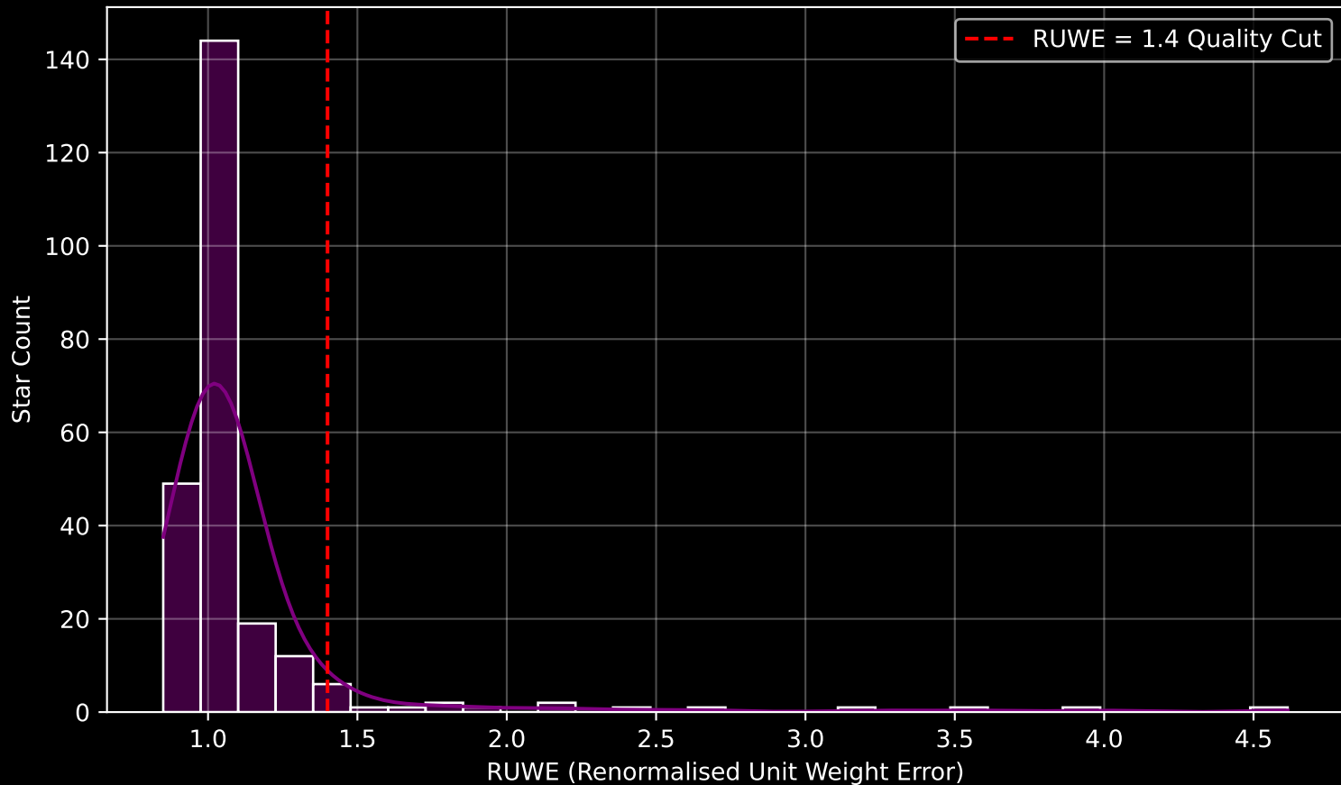
GALAH DR4 Field [1303] RUWE Distribution (n= 243)
