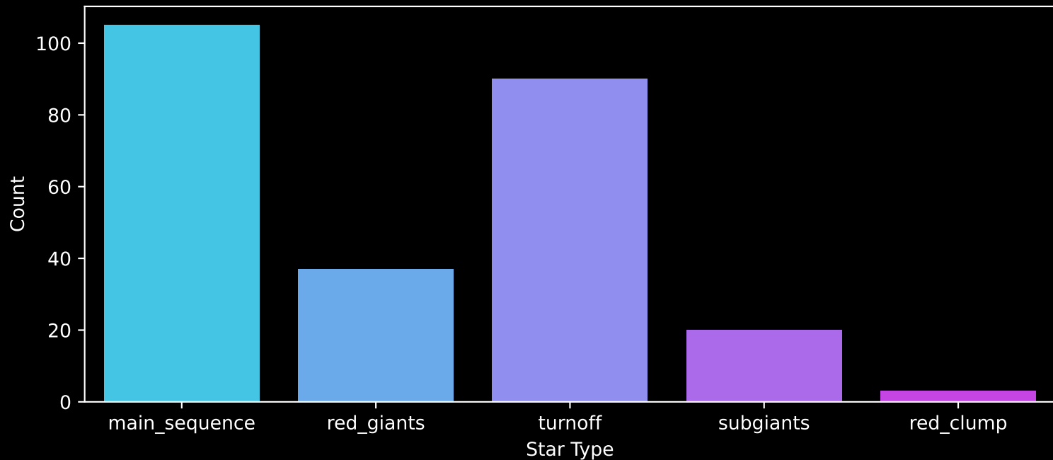
GALAH DR4 Field: [1303] Count plot of Star Type
